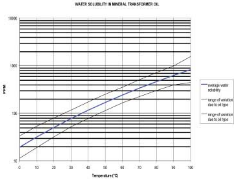
Moisture levels in oil are affected by temperature cycling of a transformer. The extent to which oil is water soluble is dependant on temperature: the more the temperature rises, the more soluble it is.
